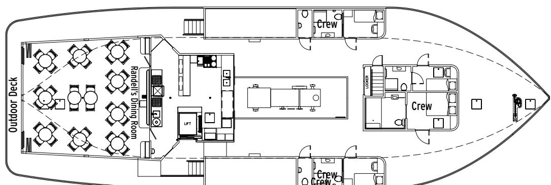
MAIN DECK
