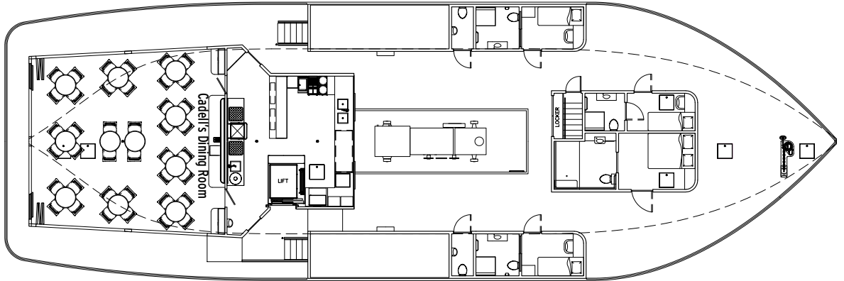
MAIN DECK
